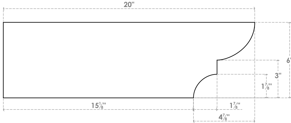
SIDE PROFILE
